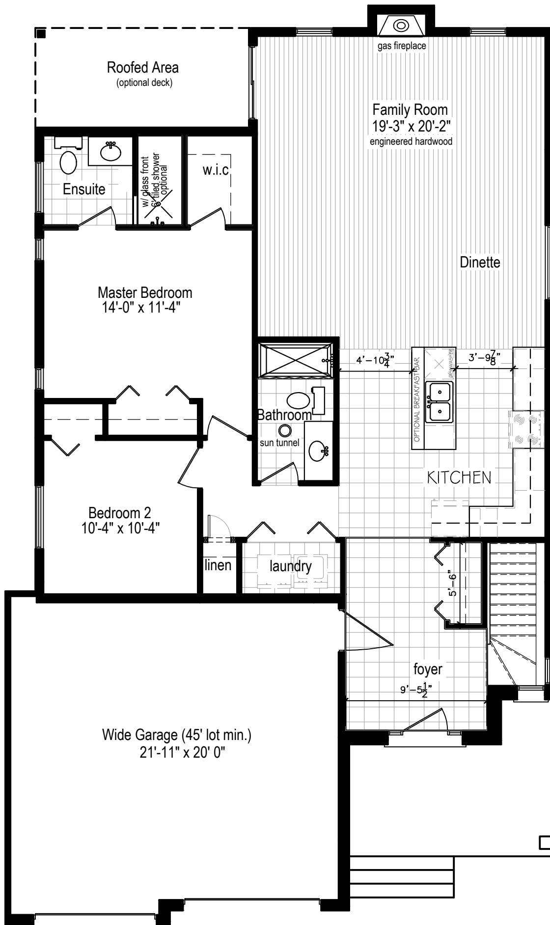
Ground Floor
